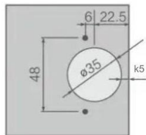
Door panel installation dimensions
