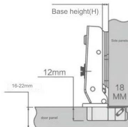
Side panel installation dimensions
