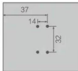
Side panel installation dimensions
